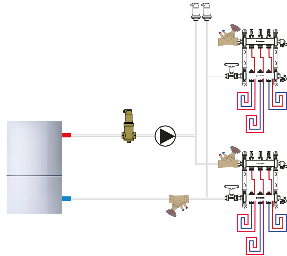
Small heat pump system with surface heating and air separator
