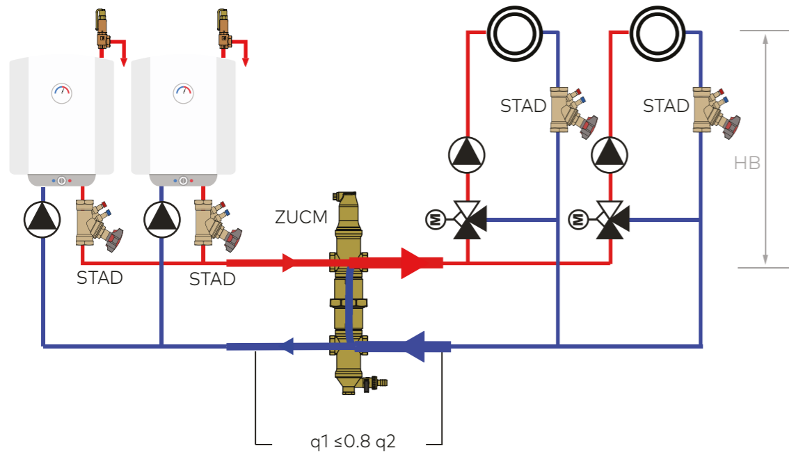
Low loss header with variable flows on the primary and secondary sides
