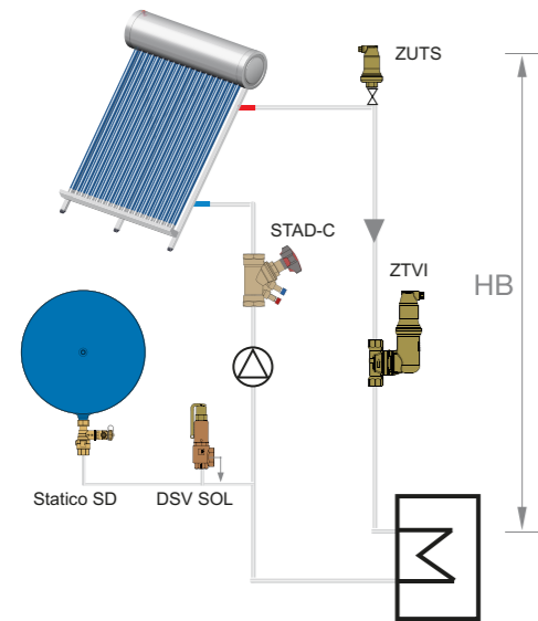
Solar system for lower temperatures
