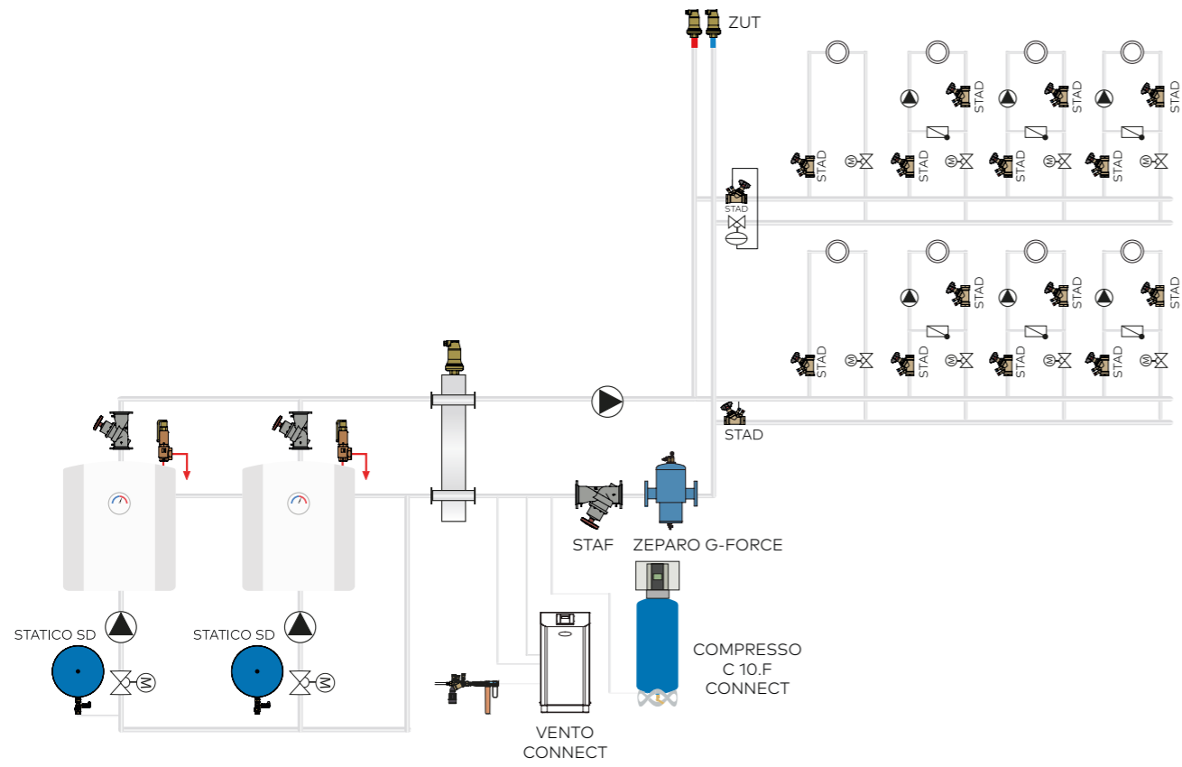
Large heating system
