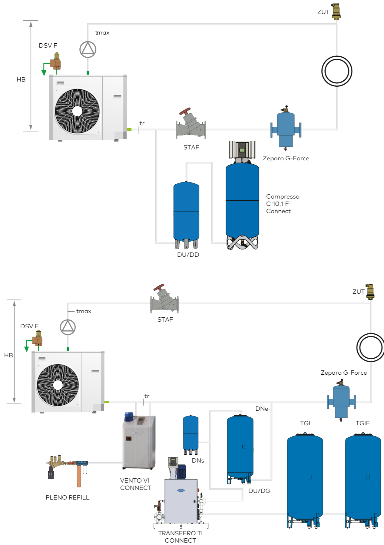
Cooling systems with chiller
