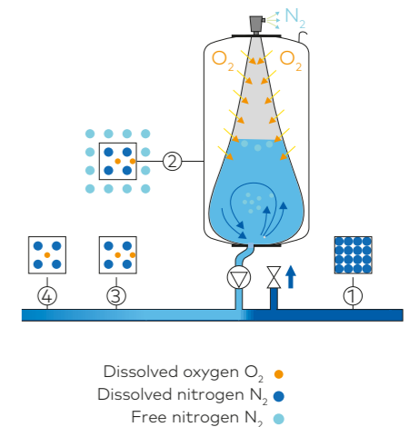
Atmospheric degassing inside the expansion vessel with oxygen diffusion through the membrane of the vessel
