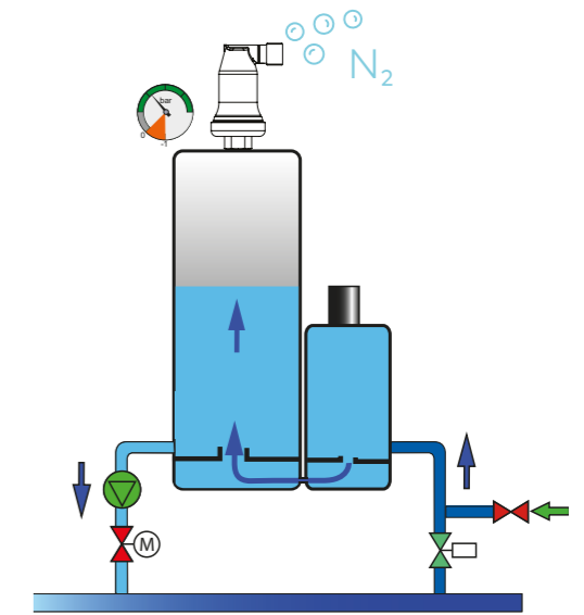
Small cyclonic vessel with tangential inlet for cyclonic gas separation
