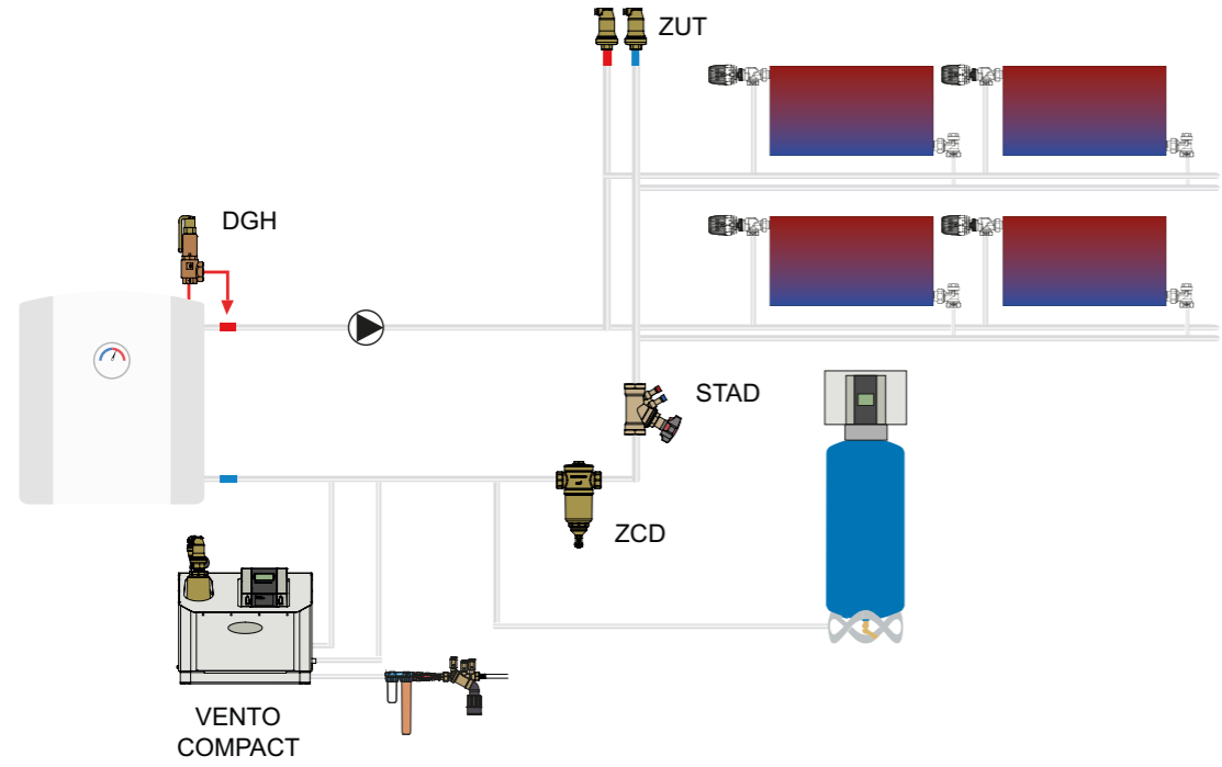
Radiator system with Statico fixed gas cushion expansion vessel Statico and vertical distribution
