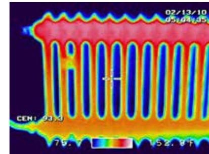
Fully vented radiator
