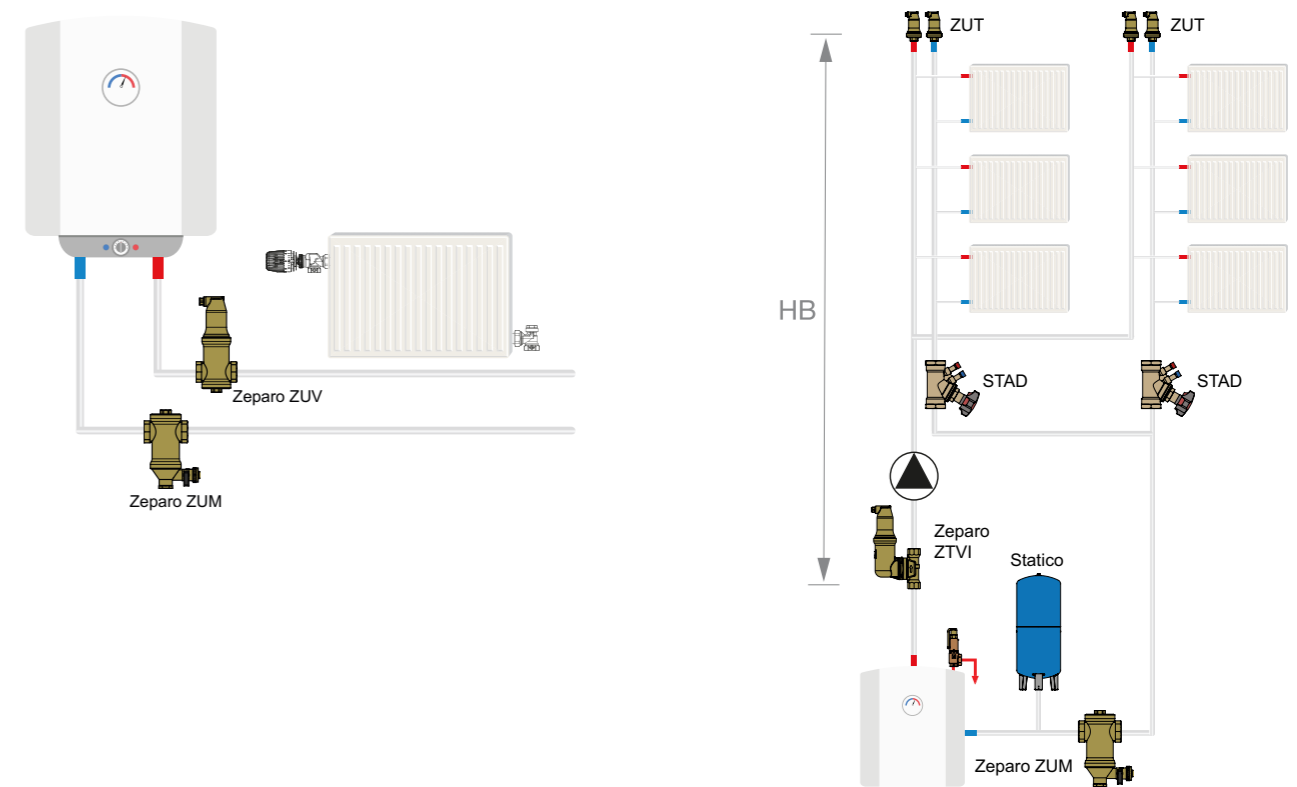
Wall-hanging gas boiler
