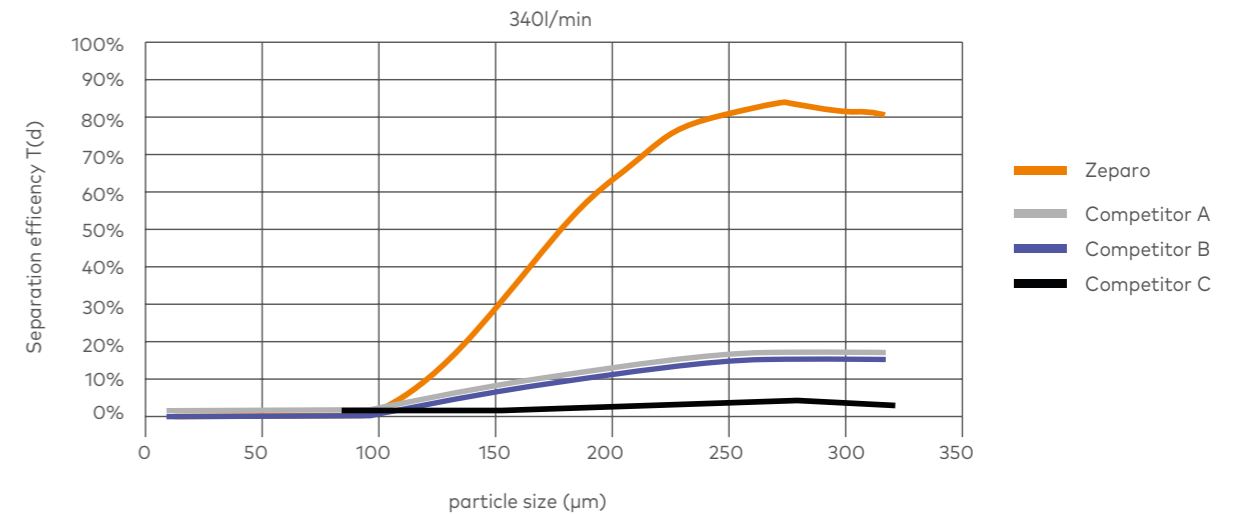
Typical separation efficiency as a function particle size in Zeparo cyclone separators compared to main competitors.
