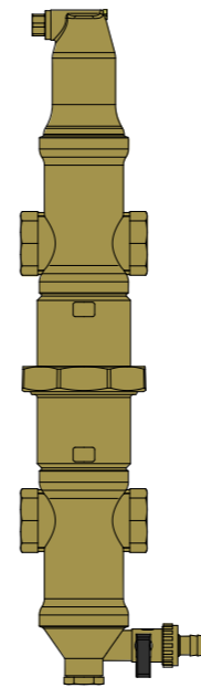
Low loss header with variable flows on the primary and secondary sides
