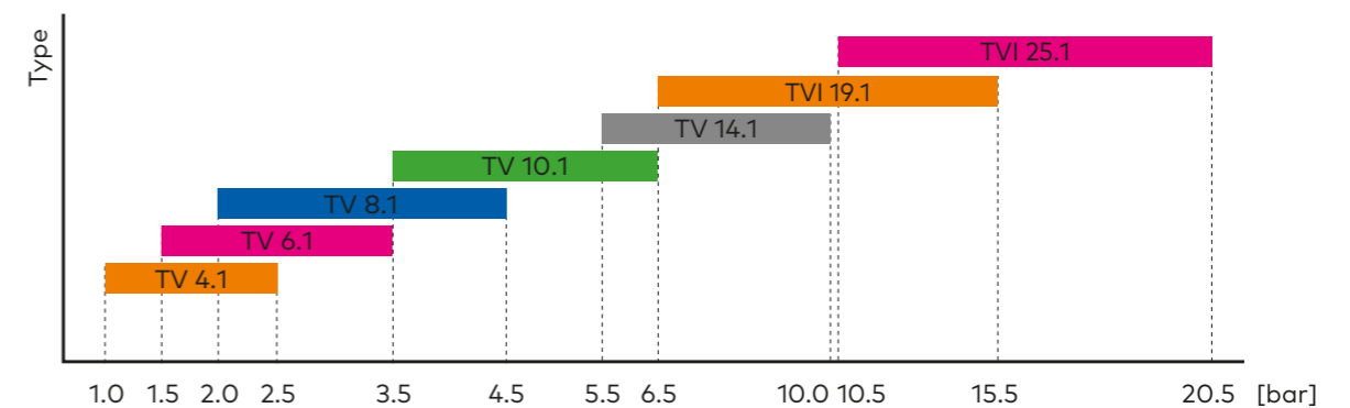
Operation range (dpu) for Pneumatex Transfero pressurisation and vacuum degassing units
