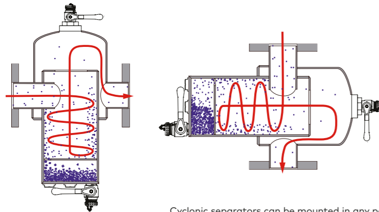
Cyclonic separators can be mounted in any position.
