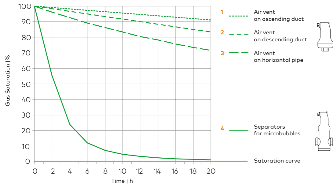
Comparison: gas saturation achievable with degassers and separators
