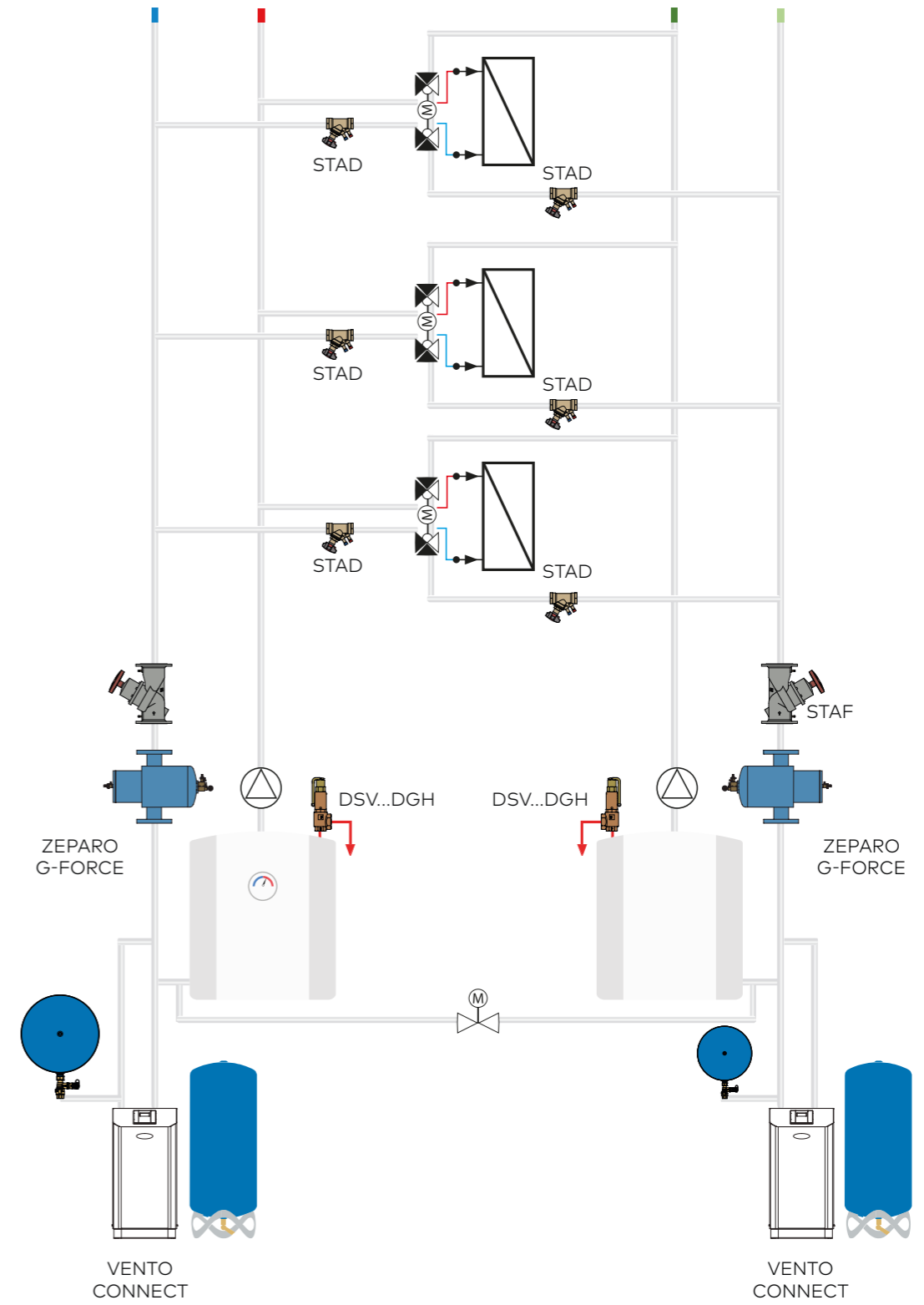
Heating/cooling system with a Transero dynamic pressurisation system and integrated vacuum degassing, which works for both heating and cooling. Automatic water content management
