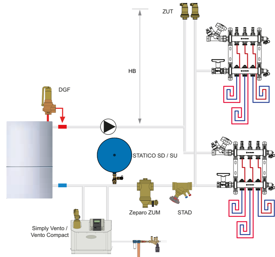
Larger Vento heat pump system with surface heating and vacuum degasser
