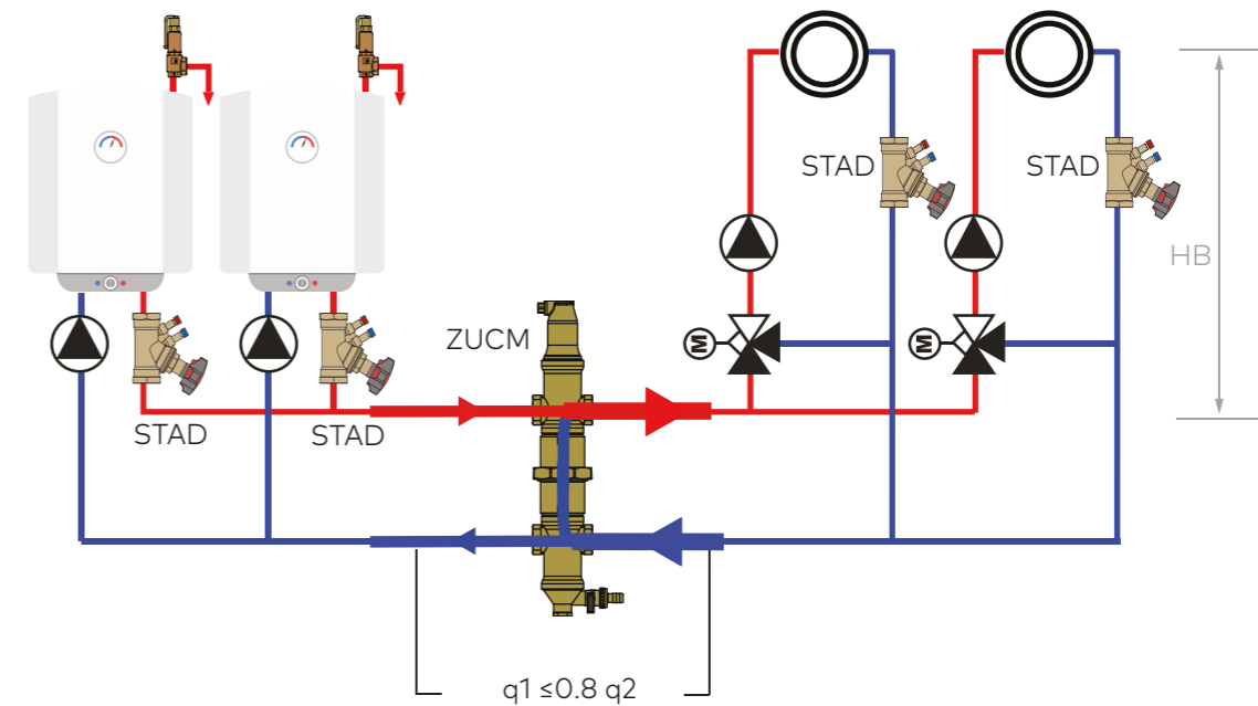
Low loss header with variable flows on the primary and secondary sides
